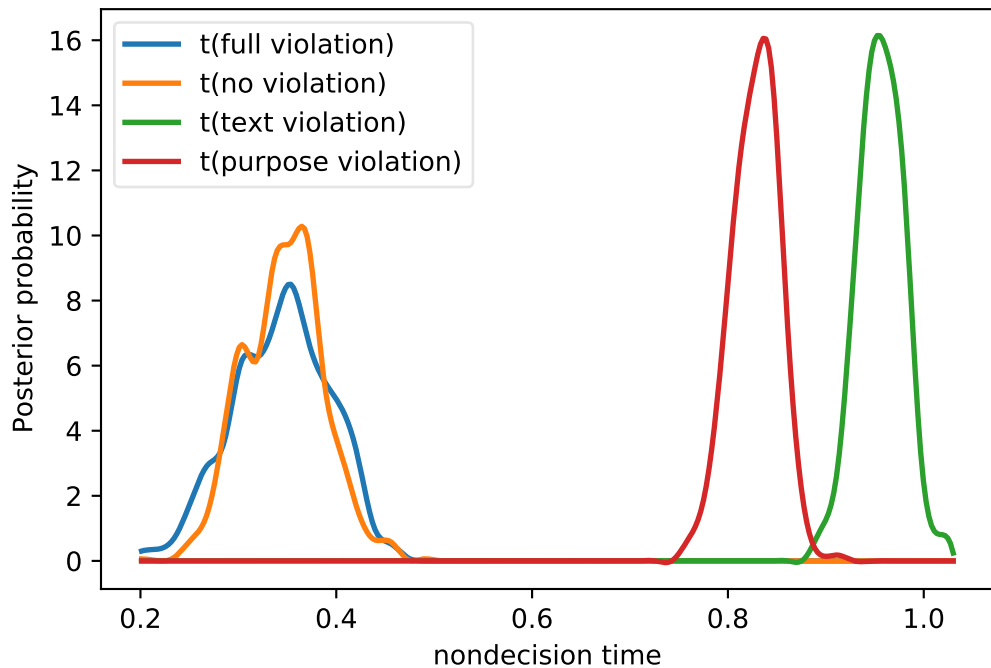
Posterior of nondecision time group means
